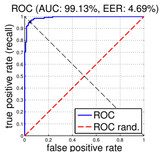
Figure 3: ROC curve of the person-independent mouthing classifier.
